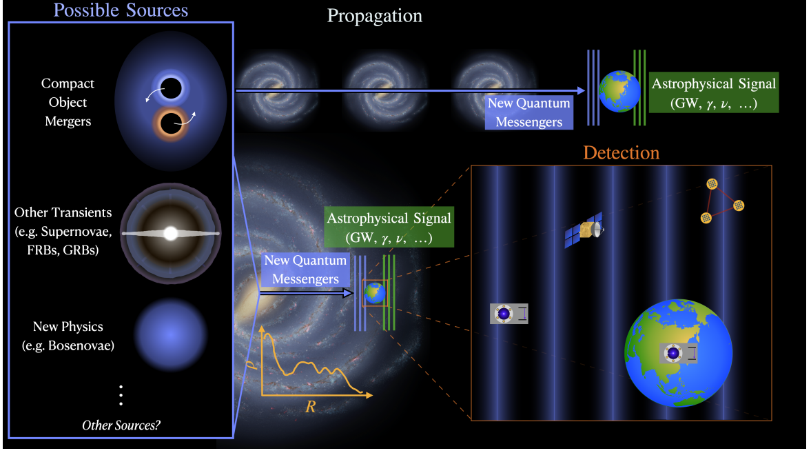
Figure 1. Illustration of multimessenger astronomy potential through synergy of astrophysical electromagnetic (photon, \gamma ), gravitational wave (GW) and neutrino ( \nu ) messengers together with ULB fields. Here, dots represent potential other astrophysical messengers, such as charged particles. Possible sources of standard astrophysical signals accompanied by relativistic bursts of ULB fields include transient astrophysical systems such as compact object (black hole, neutron star) mergers or supernovae as well as those originating from new physics beyond SM, such as boson star bosenovae. Two characteristic scenarios of messenger propagation towards detecting experiments are depicted: when sources are extragalactic (top) and fields could traverse ISM of multiple galaxies, as well as when source emission is within the Milky Way Galaxy (bottom) and fields propagate through the Galaxy’s ISM whose gas number density varying with galacto-centric distance R . Detection of ULB fields is illustrated involving terrestrial Earth-based or space-based quantum sensor experiments such as those based on precision clocks or laser/atom interferometers. ULB field signals from new physics (periwinkle shading), as well as astrophysical messenger signals (green shading) are shown. Reproduced from [36], NASA/JPL-Caltech.
