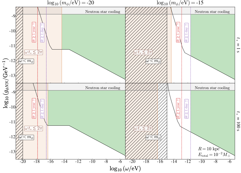
Figure 9. Sensitivity to ALP derivative coupling to neutrons, g_{\phi NN} , as a function of the ULB scalar energy \omega , considering a relativistic ULB field burst from a source located at R = 10 kpc from Earth, releasing a total energy of E_{\text{total}} = 10^{-2} M_{\odot} in the form of ULBs. Benchmark ULB masses of m_{\phi} = 10^{-20} eV (left column) and m_{\phi} = 10^{-15} eV (right column), with intrinsic burst times of t_* = 1 s (top row) and t_* = 100 s (bottom row) are displayed. The gray region represents parameter space excluded by neutron star cooling rates considering \phi production [88]. The black line shows the projected sensitivity of future experiments with g_{\text{DM}} = 10^{-11} \text{ GeV}^{-1} and t_{\text{int,DM}} = 1 day, based on proposed comagnetometers [77], electrostatic storage rings [86], NMR techniques [85], and superfluid He3 experiments [89], scaled using eq. (6.8). The black hatched and brown regions are excluded by ALP energy constraints and the uncertainty principle. Dashed purple and red lines indicate detection delays of 1 day and 1 year relative to a light-speed signal. The green region represents viable parameter space for multimessenger astronomy with ALPs, considering all constraints and benchmarks.
