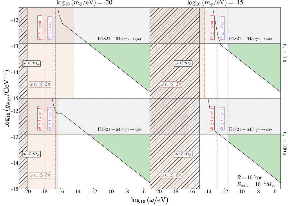
Figure 22. Sensitivity to ALP linear coupling to photons, g_{\phi\gamma\gamma} , as a function of the ULB scalar energy \omega , considering a relativistic ULB field burst from a source located at R = 10 kpc from Earth, releasing a total energy of E_{\text{total}} = 10^{-2} M_{\odot} in the form of ULBs. Benchmark ULB masses of m_{\phi} = 10^{-20} eV (left column) and m_{\phi} = 10^{-15} eV (right column), with intrinsic burst times of t_* = 1 s (top row) and t_* = 100 s (bottom row) are displayed. The gray region represents parameter space excluded by Chandra observations of spectral distortions from \gamma - \phi oscillations in luminous quasar H1821+643 [90]. The black line shows the projected sensitivity of future experiments with g_{\text{DM}} = 3 \times 10^{-16} \text{ GeV}^{-1} and t_{\text{int,DM}} = 1 year, based on proposed superconducting cavities [82] and lumped-element detectors [83], scaled using eq. (6.7). The black hatched and brown regions are excluded by ALP energy constraints and the uncertainty principle. Dashed purple and red lines indicate detection delays of 1 day and 1 year relative to a light-speed signal. The green region denotes viable parameter space for multimessenger astronomy with scalars, considering all constraints and benchmarks.
