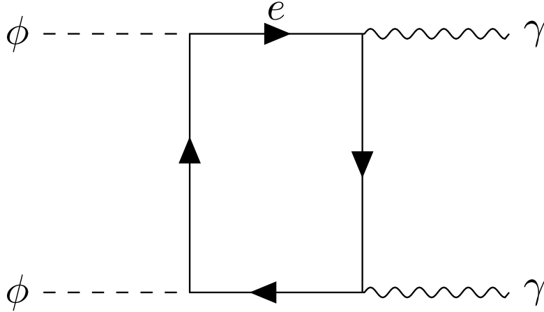
Figure 2. Induced effective quadratic ULB field coupling to photons arising from loop-level contributions of linear ULB coupling to electrons.
