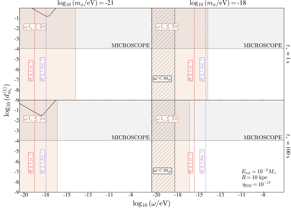
Figure 12. Sensitivity to linear dilatonic scalar coupling to electrons, d_{m_e}^{(1)} , as a function of the ULB scalar energy \omega , considering a relativistic ULB field burst from a source located at R = 10 kpc from Earth, releasing a total energy of E_{\text{total}} = 10^{-2} M_{\odot} in the form of ULBs. Benchmark ULB masses of m_{\phi} = 10^{-21} eV (left column) and m_{\phi} = 10^{-18} eV (right column), with intrinsic burst times of t_* = 1 s (top row) and t_* = 100 s (bottom row) are displayed. The gray line and shaded region indicate the parameter space excluded by MICROSCOPE EP tests [37]. The black line shows the projected sensitivity of future experiments, based on \eta_{\text{DM}} = 10^{-17} from molecular spectra analysis of SrOH [72], scaled for the scalar burst characteristics using eq. (6.5). The black hatched and brown-shaded regions are excluded due to the scalar energy being less than its mass and the uncertainty principle, respectively. Dashed purple and red lines represent detection delays of 1 day and 1 year, respectively, relative to a signal traveling at the speed of light. For the given benchmarks, no viable parameter space exists for multimessenger astronomy with scalars.
