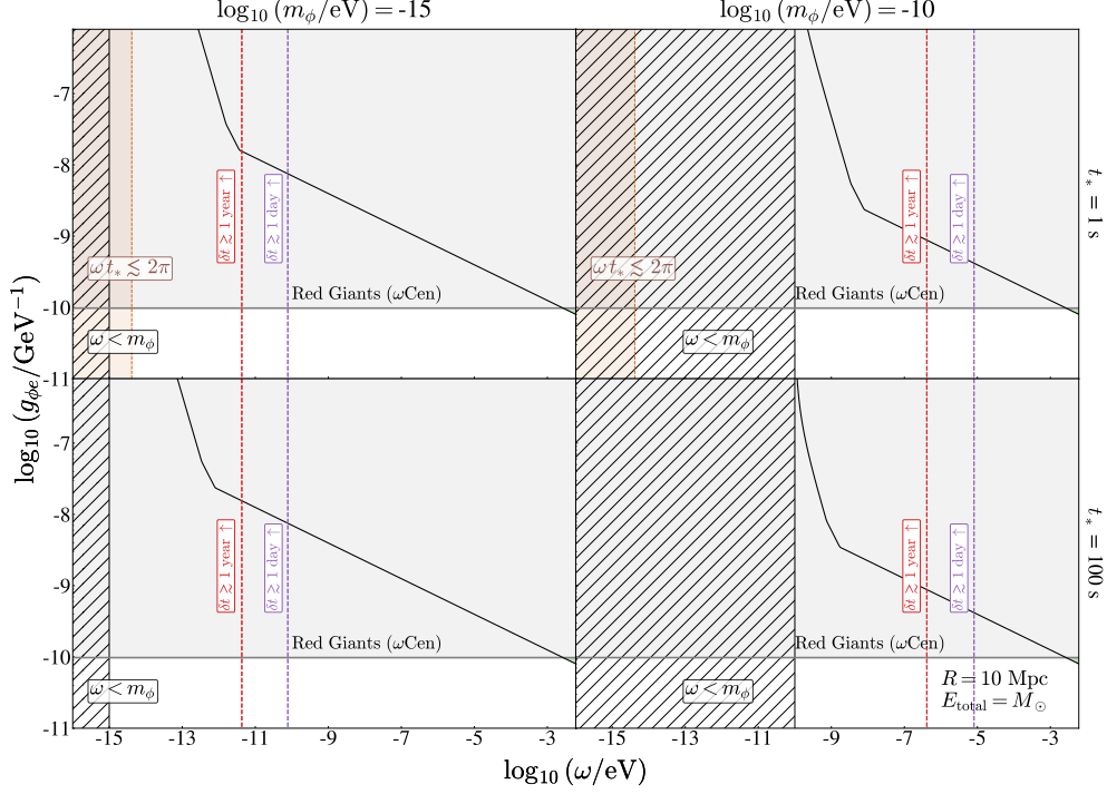
Figure 25. Sensitivity to ALP derivative coupling to electrons, g_{\phi e} , as a function of the ULB scalar energy \omega , considering a relativistic ULB field burst from a source located at R = 10 Mpc from Earth, releasing a total energy of E_{\text{total}} = M_\odot in the form of ULBs. Benchmark ULB masses of m_\phi = 10^{-15} eV (left column) and m_\phi = 10^{-10} eV (right column), with intrinsic burst times of t_* = 1 s (top row) and t_* = 100 s (bottom row) are displayed. The gray region represents parameter space excluded by cooling in tip of the red-giant branch in \omega Centauri from \phi emission [91]. The black line shows the projected sensitivity of future experiments with g_{\text{DM}} = 2 \times 10^{-11} \text{ GeV}^{-1} and t_{\text{int,DM}} = 1 year, based on proposed magnetometers [76] and torsion pendulums [78], scaled using eq. (6.8). The black hatched and brown regions are excluded by ALP energy constraints and the uncertainty principle. Dashed purple and red lines indicate detection delays of 1 day and 1 year relative to a light-speed signal. For these benchmarks, no viable parameter space exists for multimessenger astronomy with ALPs.
