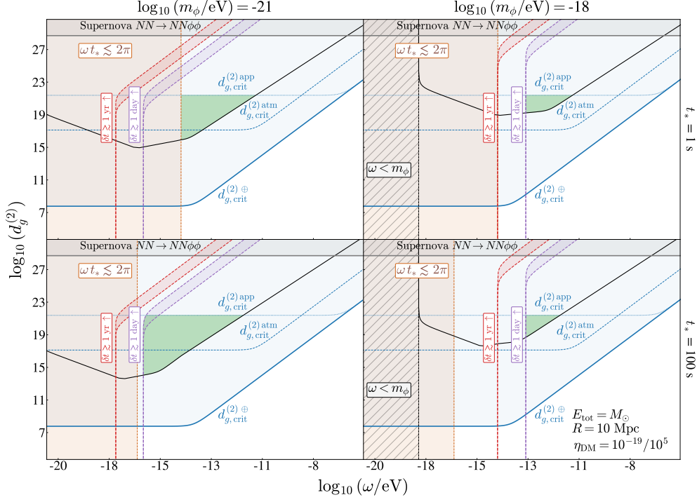
Figure 20. Sensitivity to quadratic dilatonic scalar coupling to gluons, d_g^{(2)} , as a function of the ULB scalar energy \omega , considering a relativistic ULB field burst from a source located at R = 10 Mpc from Earth, releasing a total energy of E_{\text{total}} = M_\odot in the form of ULBs. Benchmark ULB masses of m_\phi = 10^{-21} eV (left column) and m_\phi = 10^{-18} eV (right column), with intrinsic burst times of t_* = 1 s (top row) and t_* = 100 s (bottom row) are displayed. The blue solid, dashed, and dotted lines indicate critical screening from the Earth, atmosphere, and experimental apparatus, respectively. The black line shows the projected sensitivity of future experiments with \eta_{\text{DM}} = 10^{-24} , based on a Thorium isomer nuclear clock proposal [69, 71], scaled using eq. (6.6). The black hatched and brown regions are excluded by scalar energy constraints and the uncertainty principle. Dashed purple and red lines represent detection delays of 1 day and 1 year relative to a light-speed signal. The green region denotes viable parameter space for multimessenger astronomy with scalars, considering all constraints and benchmarks.
