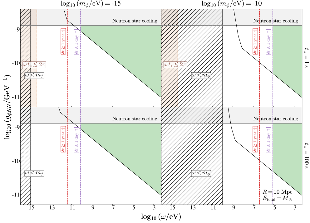
Figure 10. Sensitivity to ALP derivative coupling to neutrons, g_{\phi NN} , as a function of the ULB scalar energy \omega , considering a relativistic ULB field burst from a source located at R = 10 Mpc from Earth, releasing a total energy of E_{\text{total}} = M_{\odot} in the form of ULBs. Benchmark ULB masses of m_{\phi} = 10^{-15} eV (left column) and m_{\phi} = 10^{-10} eV (right column), with intrinsic burst times of t_* = 1 s (top row) and t_* = 100 s (bottom row) are displayed. The gray region represents parameter space excluded by neutron star cooling rates considering \phi production [88]. The black line shows the projected sensitivity of future experiments with g_{\text{DM}} = 10^{-11} \text{GeV}^{-1} and t_{\text{int,DM}} = 1 day, based on proposed comagnetometers [77], electrostatic storage rings [86], NMR techniques [85], and superfluid He3 experiments [89], scaled using eq. (6.8). The black hatched and brown regions are excluded by ALP energy constraints and the uncertainty principle. Dashed purple and red lines indicate detection delays of 1 day and 1 year relative to a light-speed signal. The green region denotes viable parameter space for multimessenger astronomy with ALPs, considering all constraints and benchmarks.
