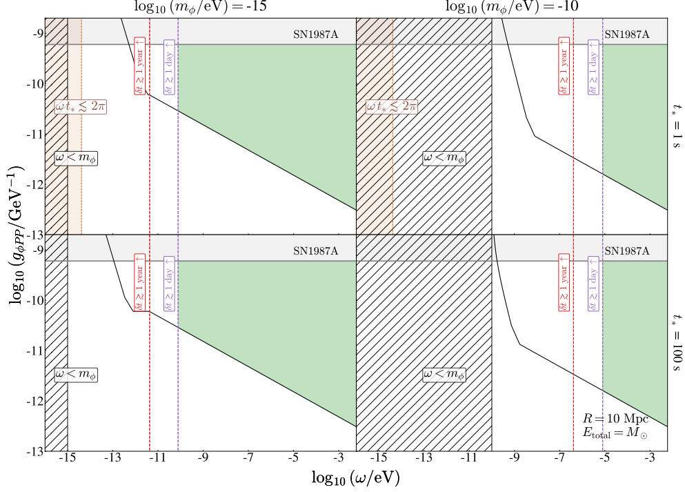
Figure 27. Sensitivity to ALP derivative coupling to protons, g_{\phi PP} , as a function of the ULB scalar energy \omega , considering a relativistic ULB field burst from a source located at R = 10 Mpc from Earth, releasing a total energy of E_{\text{total}} = M_\odot in the form of ULBs. Benchmark ULB masses of m_\phi = 10^{-15} eV (left column) and m_\phi = 10^{-10} eV (right column), with intrinsic burst times of t_* = 1 s (top row) and t_* = 100 s (bottom row) are displayed. The gray region represents parameter space excluded by ALP signals in the Kamiokande-II neutrino experiment associated with supernova SN1987A [92]. The black line shows the projected sensitivity of future experiments with g_{\text{DM}} = 10^{-12} \text{GeV}^{-1} and t_{\text{int,DM}} = 1000 s, based on proposed NMR techniques [85] and proton storage rings [84], scaled using eq. (6.8). The black hatched and brown regions are excluded by ALP energy constraints and the uncertainty principle. Dashed purple and red lines indicate detection delays of 1 day and 1 year relative to a light-speed signal. The green region represents viable parameter space for multimessenger astronomy with ALPs, considering all constraints and benchmarks.
