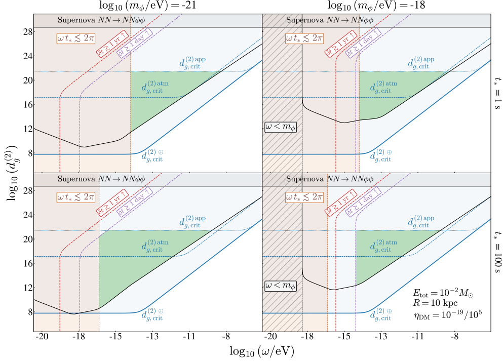
Figure 18. Sensitivity to quadratic dilatonic scalar coupling to gluons, d_g^{(2)} , as a function of the ULB scalar energy \omega , considering a relativistic ULB field burst from a source located at R = 10 kpc from Earth, releasing a total energy of E_{\text{total}} = 10^{-2} M_\odot in the form of ULBs. Benchmark ULB masses of m_\phi = 10^{-21} eV (left column) and m_\phi = 10^{-18} eV (right column), with intrinsic burst times of t_* = 1 s (top row) and t_* = 100 s (bottom row) are displayed. The blue solid, dashed, and dotted lines indicate critical screening from the Earth, atmosphere, and experimental apparatus, respectively. The black line represents the projected sensitivity of future experiments with \eta_{\text{DM}} = 10^{-24} , based on a Thorium isomer nuclear clock proposal [69, 71], scaled using eq. (6.6). The black hatched and brown regions are excluded by the requirements that scalar energy exceeds its mass and the uncertainty principle. Dashed purple and red lines show detection delays of 1 day and 1 year relative to a light-speed signal. The green region denotes the viable parameter space for multimessenger astronomy with scalars, considering all constraints and benchmarks.
