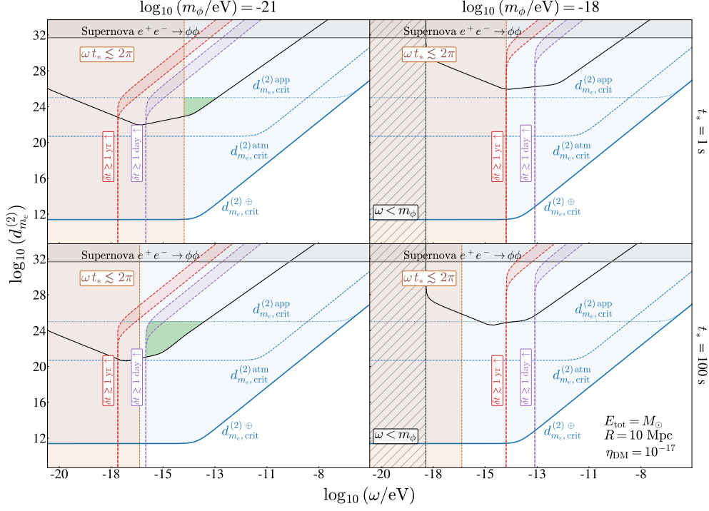
Figure 19. Sensitivity to quadratic dilatonic scalar coupling to electrons, d_{m_e}^{(2)} , as a function of the ULB scalar energy \omega , considering a relativistic ULB field burst from a source located at R = 10 Mpc from Earth, releasing a total energy of E_{\text{total}} = M_\odot in the form of ULBs. Benchmark ULB masses of m_\phi = 10^{-21} eV (left column) and m_\phi = 10^{-18} eV (right column), with intrinsic burst times of t_* = 1 s (top row) and t_* = 100 s (bottom row) are displayed. The blue solid, dashed, and dotted lines represent critical screening from the Earth, atmosphere, and experimental apparatus, respectively. The black line indicates the projected sensitivity of future experiments with \eta_{\text{DM}} = 10^{-17} , based on the SrOH molecular spectra analysis [72], scaled using eq. (6.6). The black hatched and brown regions are excluded by scalar energy limits and the uncertainty principle. Dashed purple and red lines show detection delays of 1 day and 1 year relative to a light-speed signal. The green region represents the viable parameter space for multimessenger astronomy with scalars, considering all constraints and benchmarks.
