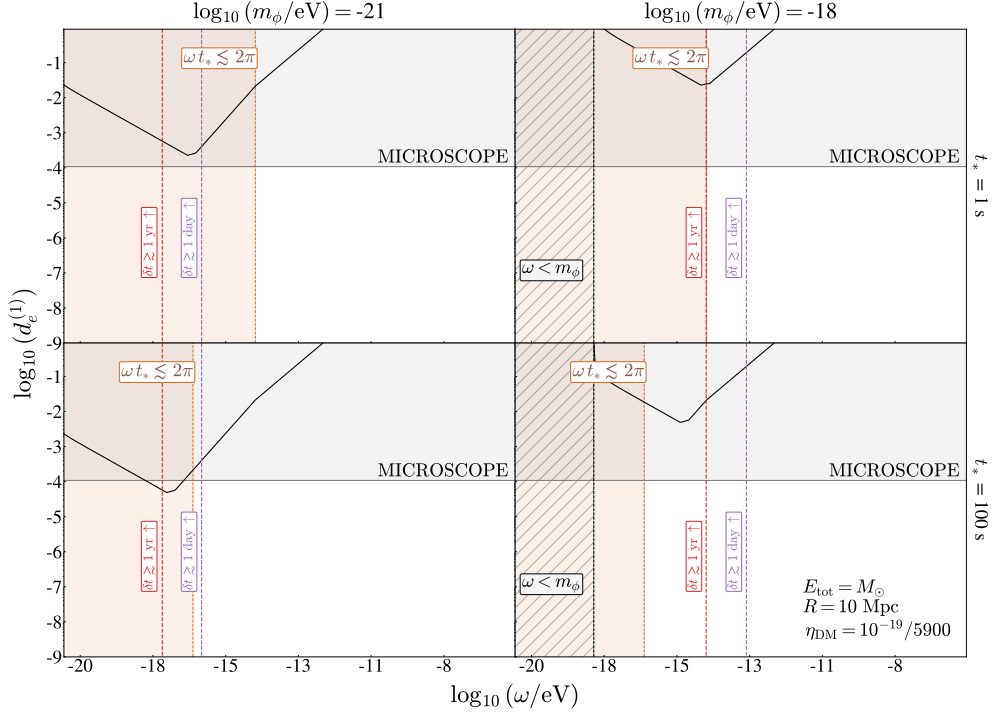
Figure 14. Sensitivity to linear dilatonic scalar coupling to photons, d_e^{(1)} , as a function of the ULB scalar energy \omega , considering a relativistic ULB field burst from a source located at R = 10 Mpc from Earth, releasing a total energy of E_{\text{total}} = M_\odot in the form of ULBs. Benchmark ULB masses of m_\phi = 10^{-21} eV (left column) and m_\phi = 10^{-18} eV (right column), with intrinsic burst times of t_* = 1 s (top row) and t_* = 100 s (bottom row) are displayed. The gray region indicates parameter space excluded by MICROSCOPE EP tests [37], and the black line represents the projected sensitivity of future experiments with \eta_{\text{DM}} = 10^{-19}/5900 , based on a Thorium isomer nuclear clock proposal [70], scaled using eq. (6.5). The black hatched and brown regions are excluded due to the scalar energy being less than its mass and the uncertainty principle, respectively. Dashed purple and red lines correspond to detection delays of 1 day and 1 year relative to a light-speed signal. For the given benchmarks, no viable parameter space exists for multimessenger astronomy with scalars.
