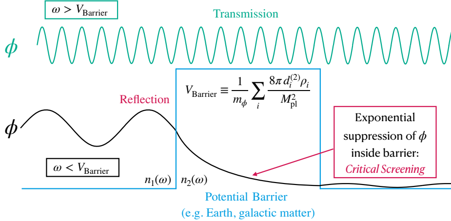
Figure 3. Schematic representation of medium (e.g. Earth, galactic matter) screening ULB wave, analogous to a finite-width potential barrier in quantum mechanics. Due to the quadratic \phi –SM coupling, a dense matter medium like Earth behaves as a potential barrier with a height V_{\text{barrier}} = \sum_i 8\pi d_i^{(2)} \rho_i / (m_\phi M_{\text{pl}}^2) . If the wave energy \omega is less than V_{\text{barrier}} , \phi primarily reflects off the barrier, with an exponentially suppressed amplitude inside. The indices of refraction, n_1(\omega) outside and n_2(\omega) inside the barrier, depend on \phi ’s energy. For \omega > V_{\text{barrier}} , the wave transmits through the barrier with reduced kinetic energy due to the increased effective mass, resulting in slower propagation.
