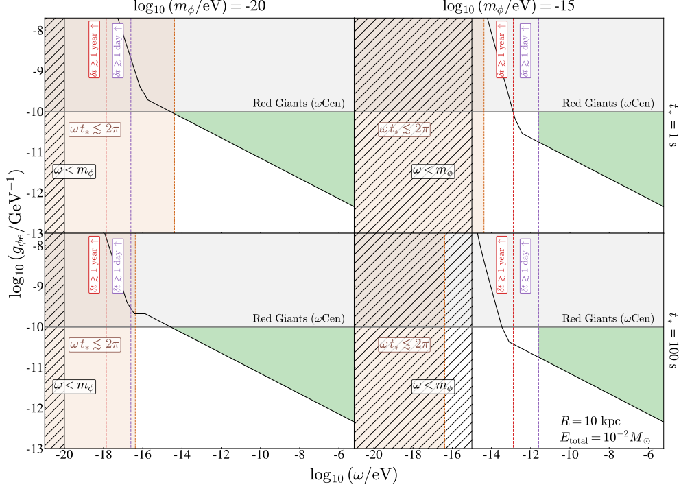
Figure 21. Sensitivity to ALP derivative coupling to electrons, g_{\phi e} , as a function of the ULB scalar energy \omega , considering a relativistic ULB field burst from a source located at R = 10 kpc from Earth, releasing a total energy of E_{\text{total}} = 10^{-2} M_{\odot} in the form of ULBs. Benchmark ULB masses of m_{\phi} = 10^{-20} eV (left column) and m_{\phi} = 10^{-15} eV (right column), with intrinsic burst times of t_* = 1 s (top row) and t_* = 100 s (bottom row) are displayed. The gray region represents parameter space excluded by cooling in tip of the red-giant branch in \omega Centauri from \phi emission [91]. The black line shows the projected sensitivity of future experiments with g_{\text{DM}} = 2 \times 10^{-11} \text{ GeV}^{-1} and t_{\text{int,DM}} = 1 year, based on proposed magnetometers [76] and torsion pendulums [78], scaled using eq. (6.8). The black hatched and brown regions are excluded due to ALP energy constraints and the uncertainty principle. Dashed purple and red lines indicate detection delays of 1 day and 1 year relative to a light-speed signal. The green region denotes viable parameter space for multimessenger astronomy with scalars, considering all constraints and benchmarks.
