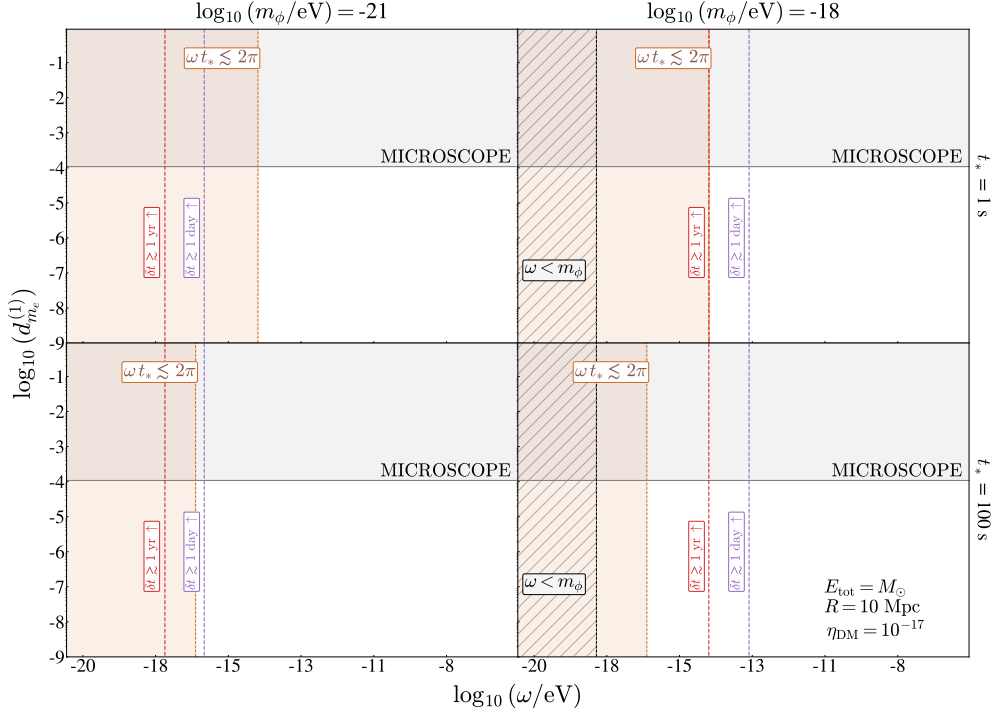
Figure 15. Sensitivity to linear dilatonic scalar coupling to electrons, d_{m_e}^{(1)} , as a function of the ULB scalar energy \omega , considering a relativistic ULB field burst from a source located at R = 10 Mpc from Earth, releasing a total energy of E_{\text{total}} = M_{\odot} in the form of ULBs. Benchmark ULB masses of m_{\phi} = 10^{-21} eV (left column) and m_{\phi} = 10^{-18} eV (right column), with intrinsic burst times of t_* = 1 s (top row) and t_* = 100 s (bottom row) are displayed. The gray region shows the parameter space excluded by MICROSCOPE EP tests [37], and the black line indicates the projected sensitivity of future experiments with \eta_{\text{DM}} = 10^{-17} , based on molecular spectra analysis of SrOH [72], scaled using eq. (6.5). The black hatched and brown regions are excluded due to the scalar energy being less than its mass and the uncertainty principle, respectively. Dashed purple and red lines represent detection delays of 1 day and 1 year relative to a light-speed signal. For the given benchmarks, no viable parameter space exists for multimessenger astronomy with scalars.
