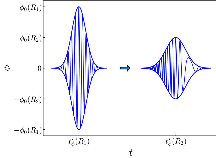
Figure 6. ULB field Gaussian wavepacket described by eq. (6.1) for a burst at two different distances, R_1 and R_2 , corresponding to elapsed times during propagation, t'_\phi(R_1) and t'_\phi(R_2) , respectively. The envelope of the wavepacket is attenuated inversely with the distance traveled R . At later times t'_\phi , the spatial extent of the ULB burst \tilde{x}_* = \tilde{t}_* increases and the oscillation frequency \omega - (2\delta\omega/\tilde{t}_*)(t - t'_\phi) exhibits chirping.
