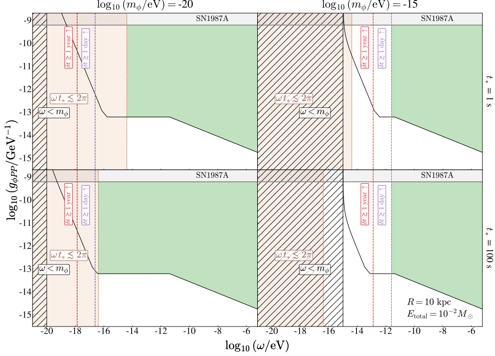
Figure 23. Sensitivity to ALP derivative coupling to protons, g_{\phi PP} , as a function of the ULB scalar energy \omega , considering a relativistic ULB field burst from a source located at R = 10 kpc from Earth, releasing a total energy of E_{\text{total}} = 10^{-2} M_{\odot} in the form of ULBs. Benchmark ULB masses of m_{\phi} = 10^{-20} eV (left column) and m_{\phi} = 10^{-15} eV (right column), with intrinsic burst times of t_* = 1 s (top row) and t_* = 100 s (bottom row) are displayed. The gray region represents parameter space excluded by ALP signals in the Kamiokande-II neutrino experiment associated with supernova SN1987A [92]. The black line shows the projected sensitivity of future experiments with g_{\text{DM}} = 10^{-12} \text{ GeV}^{-1} and t_{\text{int,DM}} = 1000 s, based on proposed NMR techniques [85] and proton storage rings [84], scaled using eq. (6.8). The black hatched and brown regions are excluded by ALP energy constraints and the uncertainty principle. Dashed purple and red lines indicate detection delays of 1 day and 1 year relative to a light-speed signal. The green region represents viable parameter space for multimessenger astronomy with ALPs, considering all constraints and benchmarks.
