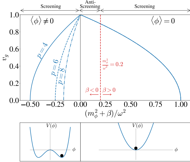
Figure 4. Group velocity of \phi waves as a function of the ratio (m_\phi^2 + \beta)/\omega^2 at V(\phi = \langle \phi \rangle) , for different choices of potential p values for \phi^p (see appendix A). Reference bare \phi field mass scenario without matter density contributions and \beta = 0 (red dashed line) delineates screening and anti-screening regimes. Schematic potential structure with respect to respective regions in the top figure is displayed on the bottom.
