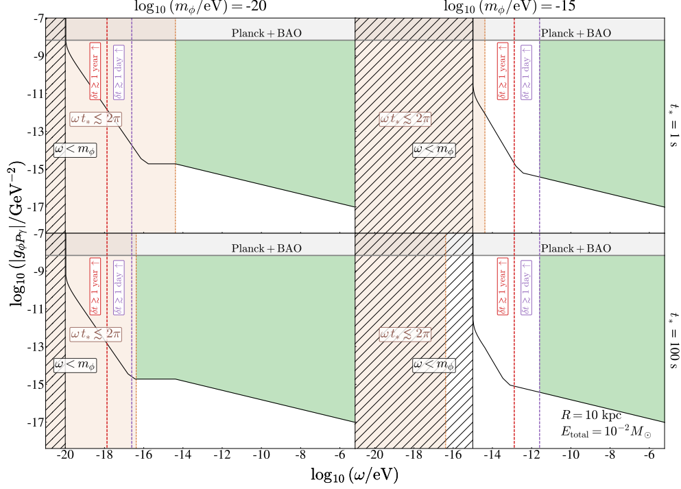
Figure 24. Sensitivity to ALP EDM coupling to protons, |g_{\phi P \gamma}| , as a function of the ULB scalar energy \omega , considering a relativistic ULB field burst from a source located at R = 10 kpc from Earth, releasing a total energy of E_{\text{total}} = 10^{-2} M_{\odot} in the form of ULBs. Benchmark ULB masses of m_{\phi} = 10^{-20} eV (left column) and m_{\phi} = 10^{-15} eV (right column), with intrinsic burst times of t_* = 1 s (top row) and t_* = 100 s (bottom row) are displayed. The gray region represents parameter space excluded by thermally-produced ALP signals in cosmic microwave background as observed by Planck2018 and baryon acoustic oscillations (BAO) data [93]. The black line shows the projected sensitivity of future experiments with g_{\text{DM}} = 10^{-18} \text{ GeV}^{-2} and t_{\text{int,DM}} = 10^6 s, based on proposed NMR techniques [85], scaled using eq. (6.7). The black hatched and brown regions are excluded by ALP energy constraints and the uncertainty principle. Dashed purple and red lines indicate detection delays of 1 day and 1 year relative to a light-speed signal. The green region denotes viable parameter space for multimessenger astronomy with ALPs, considering all constraints and benchmarks.
