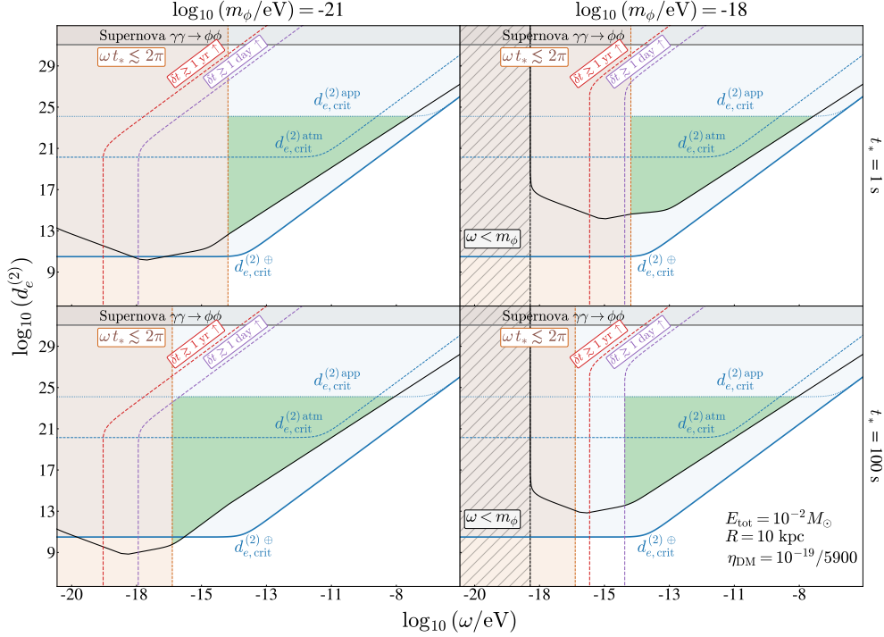
Figure 7. Sensitivity to quadratic dilatonic scalar coupling to photons, d_e^{(2)} , as a function of the ULB scalar energy \omega , considering a relativistic ULB field burst from a source located at R = 10 kpc from Earth, releasing a total energy of E_{\text{total}} = 10^{-2} M_\odot in the form of ULBs. Benchmark ULB masses of m_\phi = 10^{-21} eV (left column) and m_\phi = 10^{-18} eV (right column), with intrinsic burst times of t_* = 1 s (top row) and t_* = 100 s (bottom row) are displayed. The gray region represents parameter space excluded by direct \phi production from supernova photons [87]. The blue solid, dashed, and dotted lines indicate critical screening from the Earth, atmosphere, and experimental apparatus, respectively. The black line shows the projected sensitivity of future experiments with \eta_{\text{DM}} = 10^{-19}/5900 , based on a Thorium isomer nuclear clock proposal [70], scaled using eq. (6.6). The black hatched and brown regions are excluded due to the scalar energy being less than its mass and the uncertainty principle, respectively. Dashed purple and red lines represent detection delays of 1 day and 1 year relative to a light-speed signal. The green region denotes viable parameter space for multimessenger astronomy with scalars, given all constraints and benchmarks.
