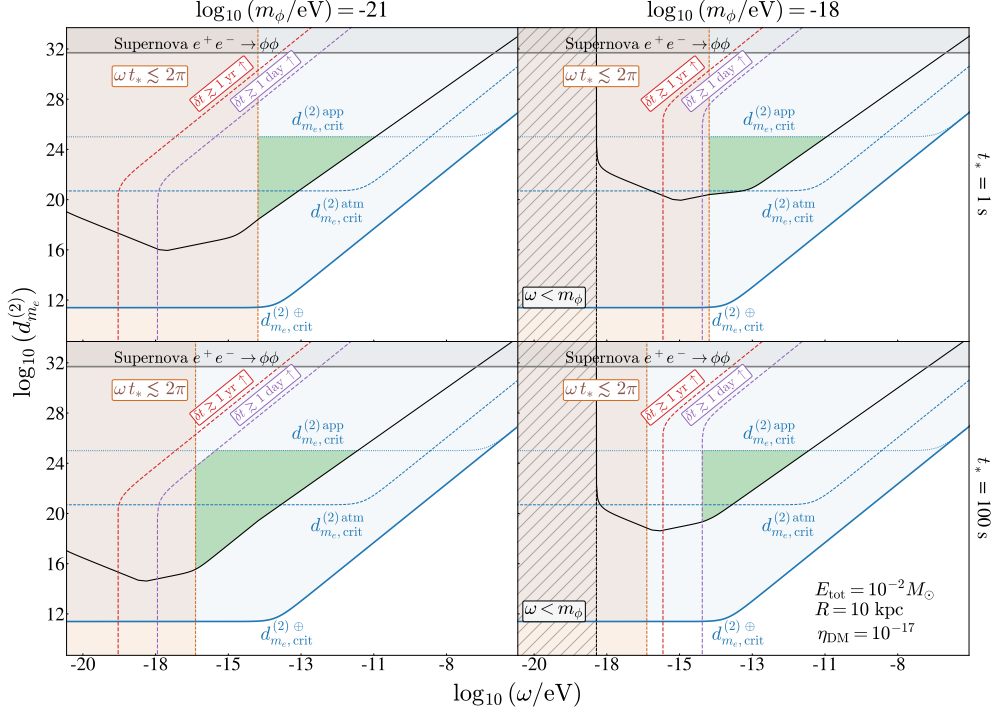
Figure 17. Sensitivity to quadratic dilatonic scalar coupling to electrons, d_{m_e}^{(2)} , as a function of the ULB scalar energy \omega , considering a relativistic ULB field burst from a source located at R = 10 kpc from Earth, releasing a total energy of E_{\text{total}} = 10^{-2} M_\odot in the form of ULBs. Benchmark ULB masses of m_\phi = 10^{-21} eV (left column) and m_\phi = 10^{-18} eV (right column), with intrinsic burst times of t_* = 1 s (top row) and t_* = 100 s (bottom row) are displayed. The blue solid, dashed, and dotted lines represent critical screening due to the Earth, atmosphere, and experimental apparatus, respectively. The black line shows the projected sensitivity of future experiments with \eta_{\text{DM}} = 10^{-17} , based on molecular spectra analysis of SrOH [72], scaled using eq. (6.6). The black hatched and brown regions are excluded due to the scalar energy being less than its mass and the uncertainty principle, respectively. Dashed purple and red lines indicate detection delays of 1 day and 1 year relative to a light-speed signal. The green region represents the viable parameter space for multimessenger astronomy with scalars, considering all constraints and benchmarks.
