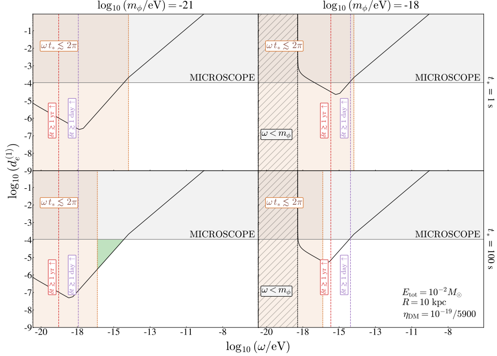
Figure 11. Sensitivity to linear dilatonic scalar coupling to photons, d_e^{(1)} , as a function of the ULB scalar energy \omega , considering a relativistic ULB field burst from a source located at R = 10 kpc from Earth, releasing a total energy of E_{\text{total}} = 10^{-2} M_{\odot} in the form of ULBs. Benchmark ULB masses of m_{\phi} = 10^{-21} eV (left column) and m_{\phi} = 10^{-18} eV (right column), with intrinsic burst times of t_* = 1 s (top row) and t_* = 100 s (bottom row) are displayed. The gray line and shaded region indicate the parameter space excluded by MICROSCOPE EP tests [37]. The black line shows the projected sensitivity of future experiments, based on \eta_{\text{DM}} = 10^{-19}/5900 , consistent with a Thorium isomer nuclear clock expectation [70], scaled for the scalar burst characteristics using eq. (6.5). The black hatched and brown-shaded regions are excluded due to the scalar energy being less than its mass and the uncertainty principle, respectively. Dashed purple and red lines represent detection delays of 1 day and 1 year, respectively, relative to a signal traveling at the speed of light. The green shaded region denotes the viable parameter space for multimessenger astronomy with scalars, considering all constraints and the given burst benchmarks.
