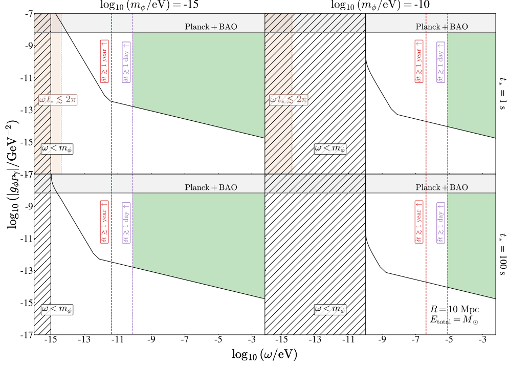
Figure 28. Sensitivity to ALP EDM coupling to protons, |g_{\phi P \gamma}| , as a function of the ULB scalar energy \omega , considering a relativistic ULB field burst from a source located at R = 10 Mpc from Earth, releasing a total energy of E_{\text{total}} = M_{\odot} in the form of ULBs. Benchmark ULB masses of m_{\phi} = 10^{-15} eV (left column) and m_{\phi} = 10^{-10} eV (right column), with intrinsic burst times of t_* = 1 s (top row) and t_* = 100 s (bottom row) are displayed. The gray region represents parameter space excluded by thermally-produced ALP signals in cosmic microwave background as observed by Planck2018 and baryon acoustic oscillations (BAO) data [93]. The black line shows the projected sensitivity of future experiments with g_{\text{DM}} = 10^{-18} \text{ GeV}^{-2} and t_{\text{int,DM}} = 10^6 s, based on proposed NMR techniques [85], scaled using eq. (6.7). The black hatched and brown regions are excluded by ALP energy constraints and the uncertainty principle. Dashed purple and red lines indicate detection delays of 1 day and 1 year relative to a light-speed signal. The green region denotes viable parameter space for multimessenger astronomy with ALPs, considering all constraints and benchmarks.
