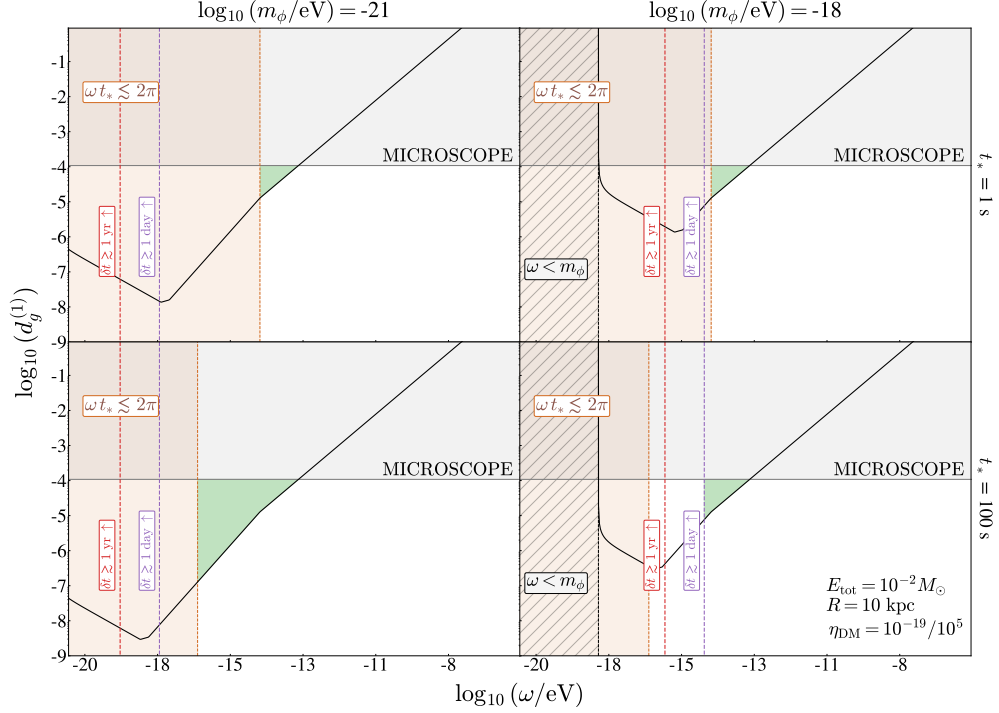
Figure 13. Sensitivity to linear dilaton scalar coupling to gluons, d_g^{(1)} , as a function of the ULB scalar energy \omega , considering a relativistic ULB field burst from a source located at R = 10 kpc from Earth, releasing a total energy of E_{\text{total}} = 10^{-2} M_\odot in the form of ULBs. Benchmark ULB masses of m_\phi = 10^{-21} eV (left column) and m_\phi = 10^{-18} eV (right column), with intrinsic burst times of t_* = 1 s (top row) and t_* = 100 s (bottom row) are displayed. The gray line and shaded region show the parameter space excluded by MICROSCOPE EP tests [37]. The black line represents the projected sensitivity of future experiments, based on \eta_{\text{DM}} = 10^{-24} , consistent with a Thorium isomer nuclear clock proposal [69, 71], scaled for the scalar burst characteristics using eq. (6.5). The black hatched and brown shaded regions are excluded due to the scalar energy being less than its mass and the uncertainty principle, respectively. Dashed purple and red lines indicate detection delays of 1 day and 1 year, respectively, relative to a signal traveling at the speed of light. The green shaded region represents the viable parameter space for multimessenger astronomy with scalars, considering all constraints and the given benchmarks.
