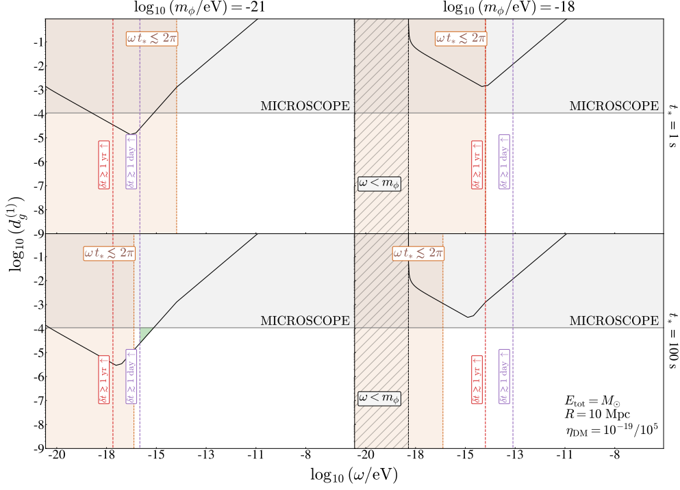
Figure 16. Sensitivity to linear dilatonic scalar coupling to gluons, d_g^{(1)} , as a function of the ULB scalar energy \omega , considering a relativistic ULB field burst from a source located at R = 10 Mpc from Earth, releasing a total energy of E_{\text{total}} = M_\odot in the form of ULBs. Benchmark ULB masses of m_\phi = 10^{-21} eV (left column) and m_\phi = 10^{-18} eV (right column), with intrinsic burst times of t_* = 1 s (top row) and t_* = 100 s (bottom row) are displayed. The gray region represents the parameter space excluded by MICROSCOPE EP tests [37], and the black line indicates the projected sensitivity of future experiments with \eta_{\text{DM}} = 10^{-24} , based on a Thorium isomer nuclear clock proposal [69, 71], scaled using eq. (6.5). The black hatched and brown regions are excluded due to the scalar energy being less than its mass and the uncertainty principle, respectively. Dashed purple and red lines correspond to detection delays of 1 day and 1 year relative to a light-speed signal. The green region indicates the viable parameter space for multimessenger astronomy with scalars, given all constraints and benchmarks.
