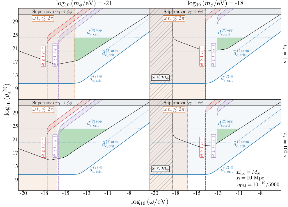
Figure 8. Sensitivity to quadratic dilaton scalar coupling to photons, d_e^{(2)} , as a function of the ULB scalar energy \omega , considering a relativistic ULB field burst from a source located at R = 10 Mpc from Earth, releasing a total energy of E_{\text{total}} = M_\odot in the form of ULBs. Benchmark ULB masses of m_\phi = 10^{-21} eV (left column) and m_\phi = 10^{-18} eV (right column), with intrinsic burst times of t_* = 1 s (top row) and t_* = 100 s (bottom row) are displayed. The gray region represents parameter space excluded by direct \phi production from supernova photons [87]. Blue solid, dashed, and dotted lines show critical screening from the Earth, atmosphere, and experimental apparatus, respectively. The black line indicates the projected sensitivity of future experiments with \eta_{\text{DM}} = 10^{-19}/5900 , based on a Thorium isomer nuclear clock proposal [70], scaled using eq. (6.6). The black hatched and brown regions are excluded by scalar energy limits and the uncertainty principle. Dashed purple and red lines represent detection delays of 1 day and 1 year relative to a light-speed signal. The green region denotes viable parameter space for multimessenger astronomy with scalars, considering all constraints and benchmarks.
