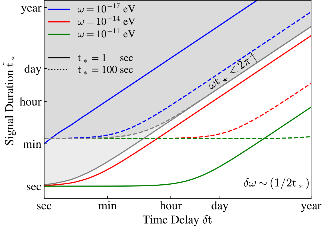
Figure 5. Duration of the signal at the detector, \tilde{t}_* , as a function of the time delay, \delta t . Different benchmarks for energy and intrinsic burst duration are shown, distinguished by colors and linestyles, respectively. The gray shaded region is excluded by the uncertainty principle relating the intrinsic burst duration and the energy of the emitted ULBs. All curves assume the minimal uncertainty case, \delta\omega = 1/(2t_*) . For larger \delta\omega , the nonzero-slope portions of the curves would shift upward linearly.
