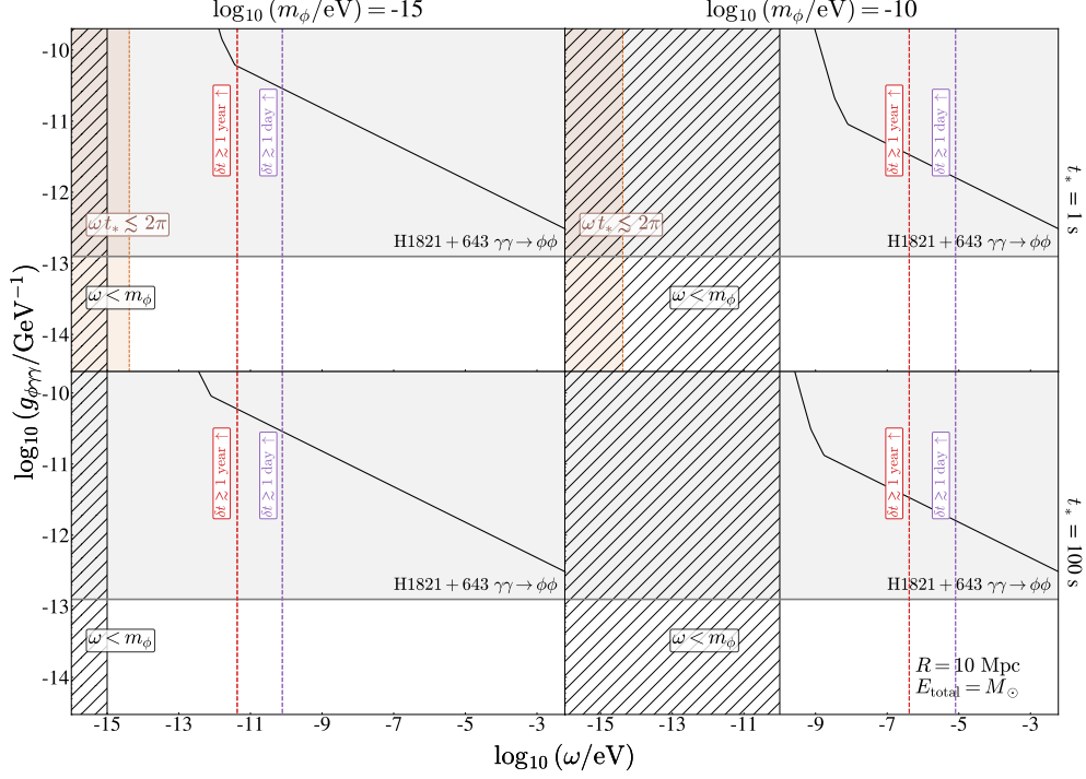
Figure 26. Sensitivity to ALP linear coupling to photons, g_{\phi\gamma\gamma} , as a function of the ULB scalar energy \omega , considering a relativistic ULB field burst from a source located at R = 10 Mpc from Earth, releasing a total energy of E_{\text{total}} = M_\odot in the form of ULBs. Benchmark ULB masses of m_\phi = 10^{-15} eV (left column) and m_\phi = 10^{-10} eV (right column), with intrinsic burst times of t_* = 1 s (top row) and t_* = 100 s (bottom row) are displayed. The gray region represents parameter space excluded by Chandra observations of spectral distortions from \gamma - \phi oscillations in luminous quasar H1821+643 [90]. The black line shows the projected sensitivity of future experiments with g_{\text{DM}} = 3 \times 10^{-16} \text{GeV}^{-1} and t_{\text{int,DM}} = 1 year, based on proposed superconducting cavities [82] and lumped-element detectors [83], scaled using eq. (6.7). The black hatched and brown regions are excluded by ALP energy constraints and the uncertainty principle. Dashed purple and red lines indicate detection delays of 1 day and 1 year relative to a light-speed signal. For these benchmarks, no viable parameter space exists for multimessenger astronomy with ALPs.
